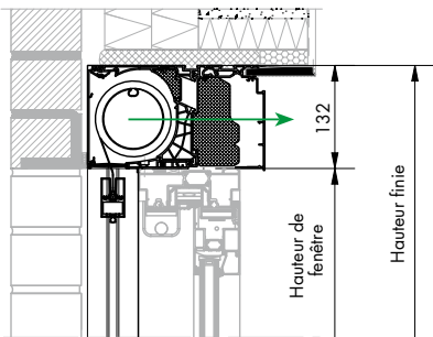
Situation de montage 4: Fixscreen® Mono AK EVO Large
