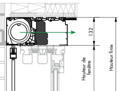
Situation de montage 4: Fixscreen® Mono AK EVO XX-Large
