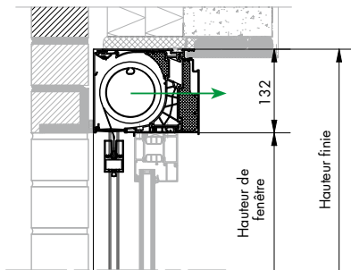
Situation de montage 4: Fixscreen® Mono AK EVO Small
