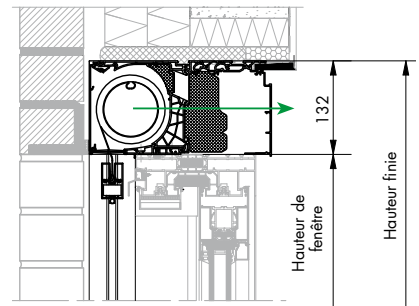
Situation de montage 4: Fixscreen® Mono AK EVO X-Large
