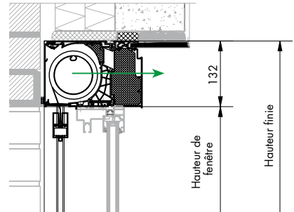
Situation de montage 4: Fixscreen® Mono AK EVO Medium
